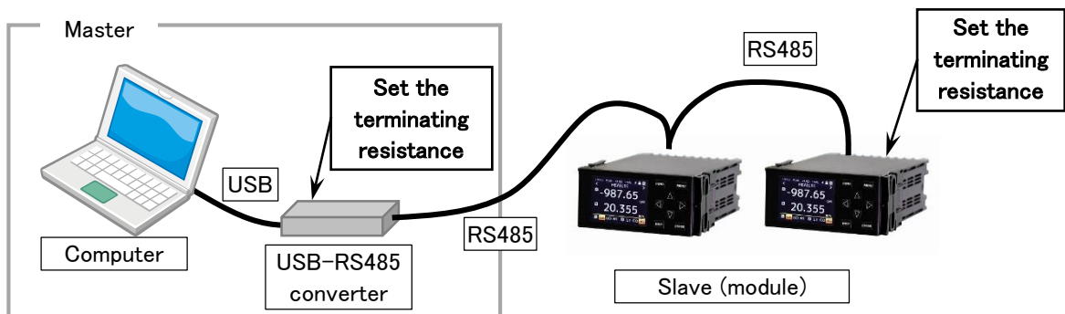
Figure 2.3 Terminating resistance when USB-RS 485 converter is used
