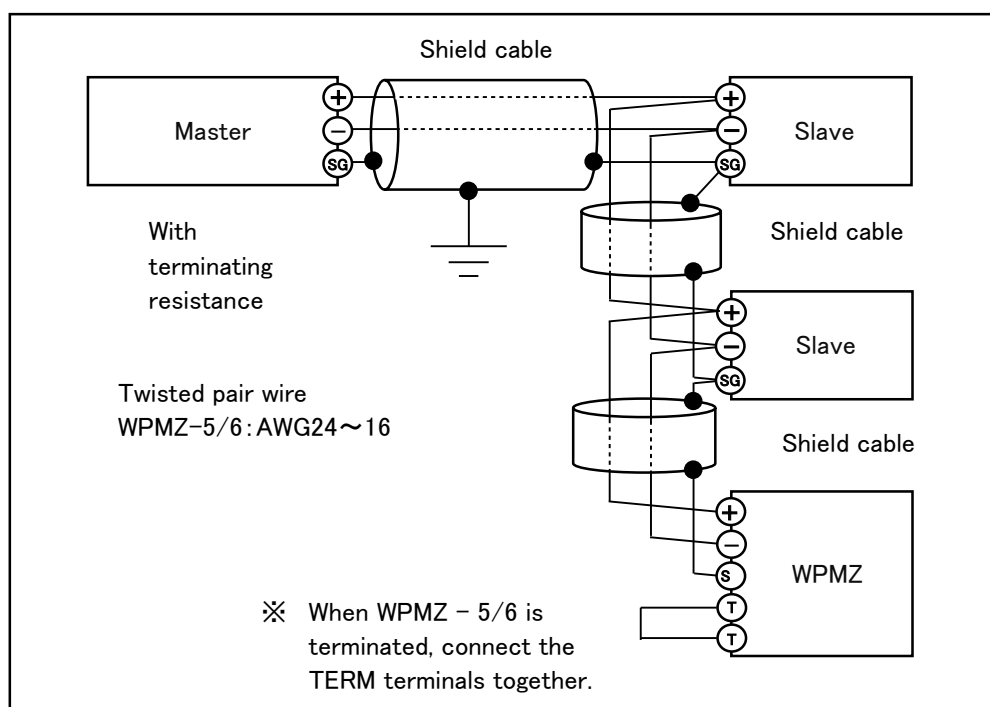
Figure 2.4 Modbus connection of WPMZ-5/6
