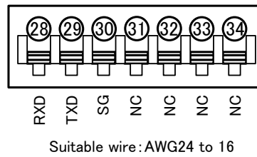
Figure 2.5 Wiring of RS-232C communication
