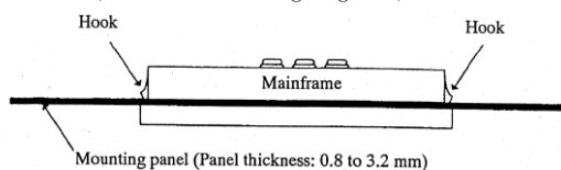
Mounting diagram
